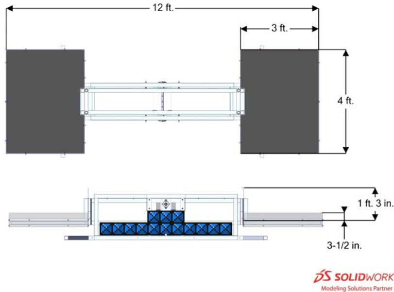
Figure 3-15: SWITCH range of motion
