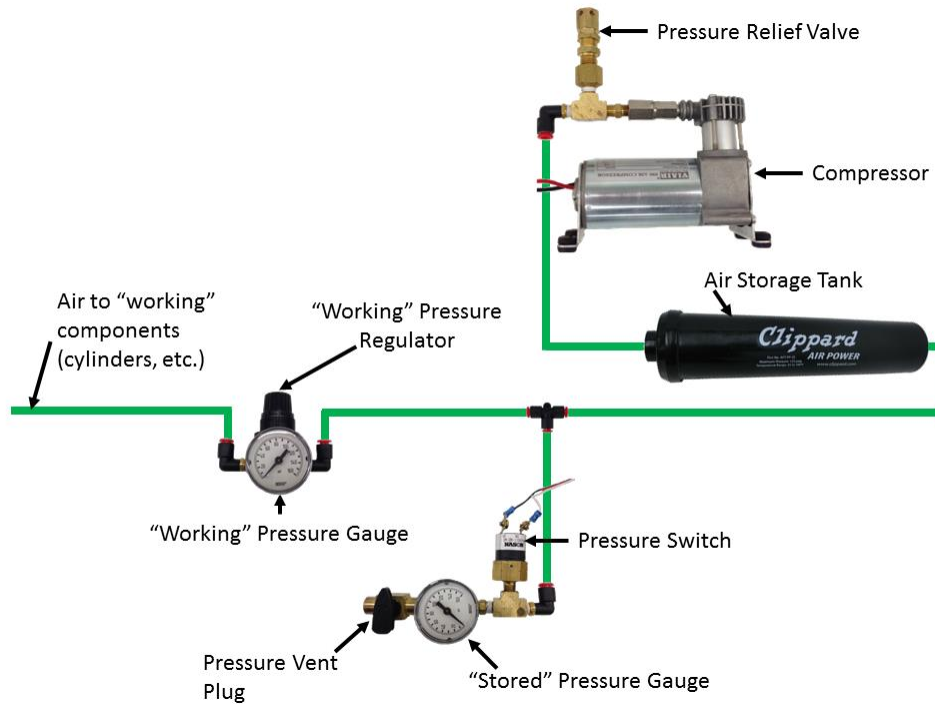
Figure 10-14 Pneumatic circuitry
